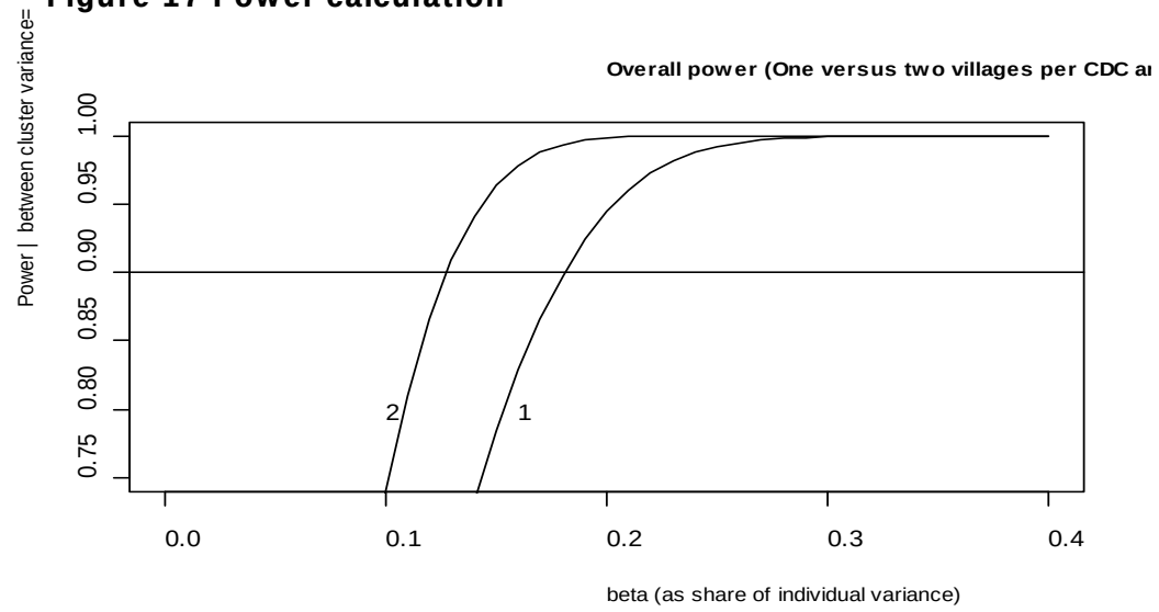
Figure 17 Power calculation
