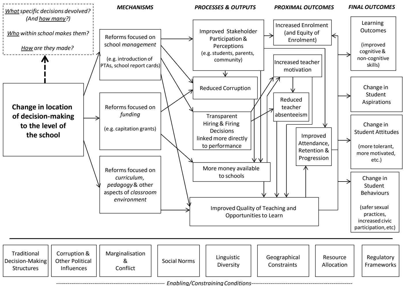
Figure 1: Conceptual framework
