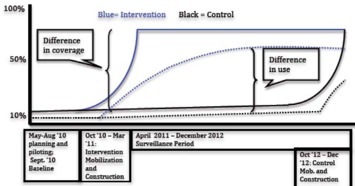
Figure 3: Implementation timeline
