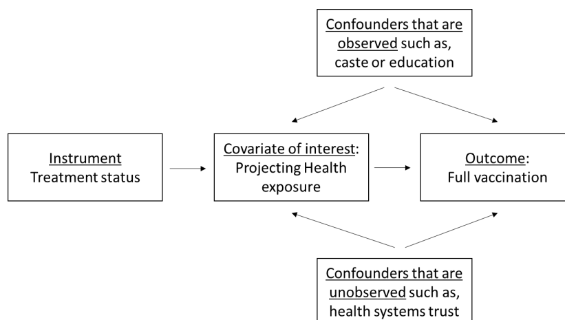
Figure 4: Schematic of instrumental variable analysis
